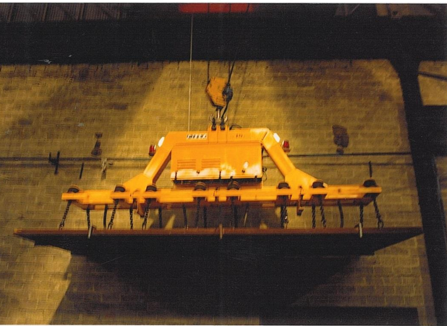
Small Vaccum lifter: 1 T & 500 Kg
